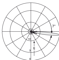
Vertical Pattern 0.5°–10° electr. downtilt
