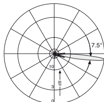
Vertical Pattern 2°–10° electrical downtilt
