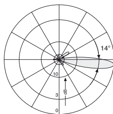
Vertical Pattern 0.5°–12° electr. downtilt
