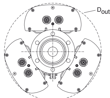
Bottom view without downtilt kit
