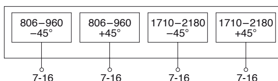
806–960 +45°/–45° Polarization
