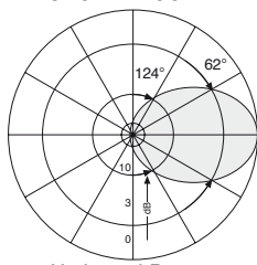
Horizontal Pattern
