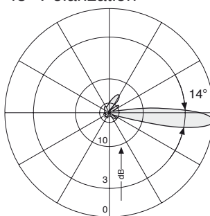
Vertical Pattern 0°–10° electrical downtilt continuously adjustable
