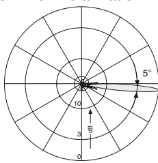
Vertical Pattern 0°–10° electrical downtilt
