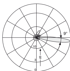
Vertical Pattern 0°–10° electr. downtilt
